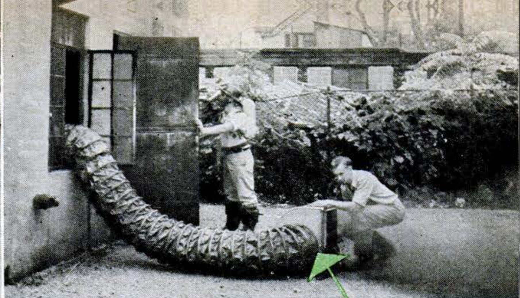
SMOKE-EATING CATERPILLAR , a new device called an ejector, clears air in seconds so firemen can enter a burning building. It is an exhaust fan on a bellows-like tube.
